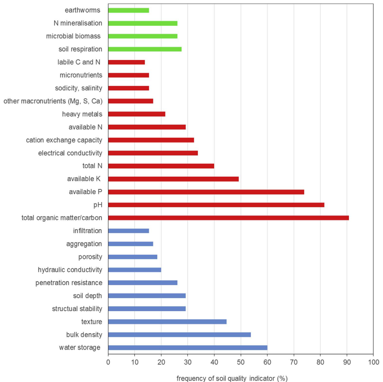
Figure 6 Frequency of use of indicators in soil quality studies (from Bünemann et al. 2018)
